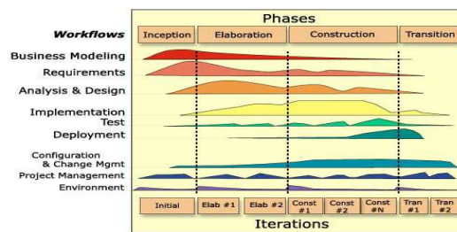
Figure 2 - Two Dimensions of the RUP
